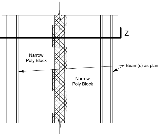
JF121 - Staggered Bearing Loadbearing Wall
