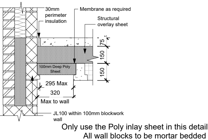
JF111 - Poly Sheet Edge Detail
