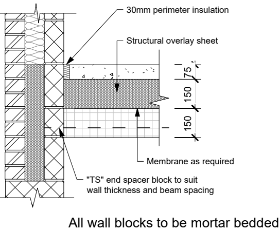
JF120 - Bearing End Detail
