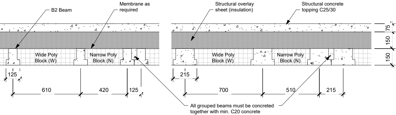
JF111 - Poly Sheet Edge Detail
